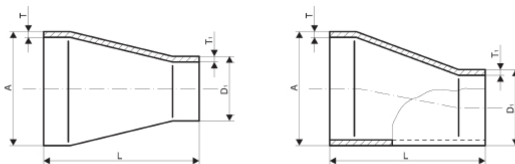
Reducers concentric and excentric according to EN 10253-1:1999 Form 2
