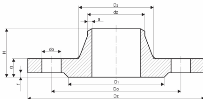
Neck flanges according to DIN 2633
