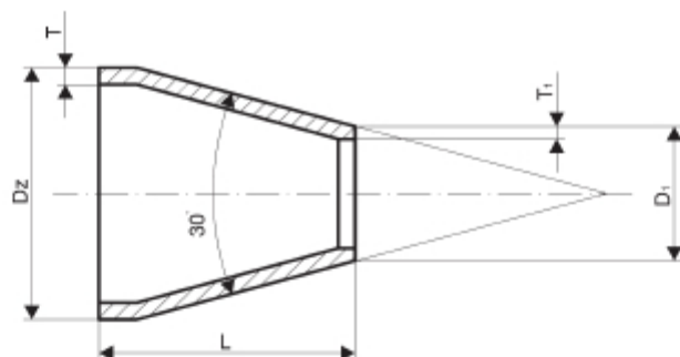
Reducers concentric according to EN 10253-1:1999 Form 1
