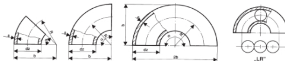
Elbows according to ANSI B16.9 type LR
