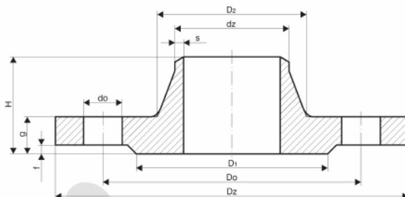
Neck flanges according to DIN 2631
