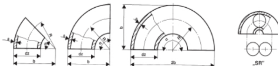
Elbows according to ANSI B16.9 type SR
