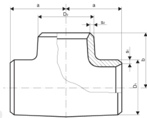
Tees according to ANSI B16.9
