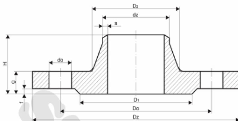
Neck flanges according to DIN 2635
