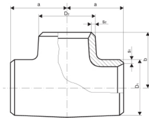
Tees according to DIN 2615-1
