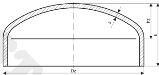
Caps according to DIN 2617
