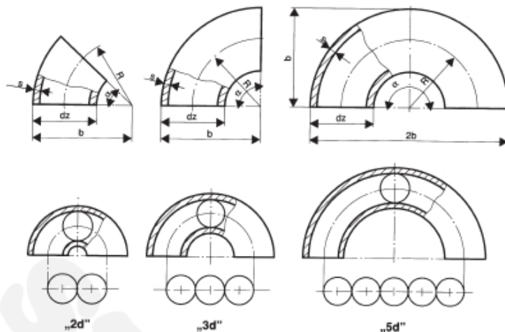
Elbows according to DIN 2605-1
