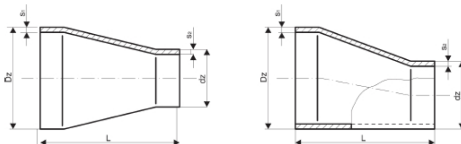
Reducers according to ANSI B16.9
