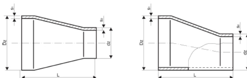
Reducers according to DIN 2616
